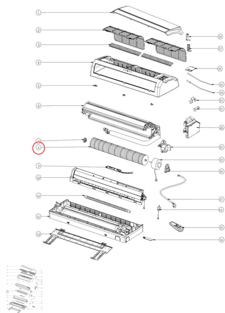
Turbina DIE/MAE 45 Airwell, Johnson y Electra. (453082400)
