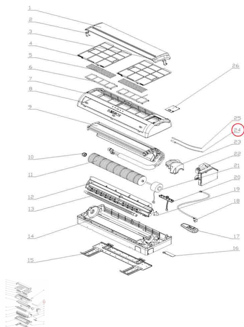
Sonda Bateria standar Airwell Johnson (4519813)
